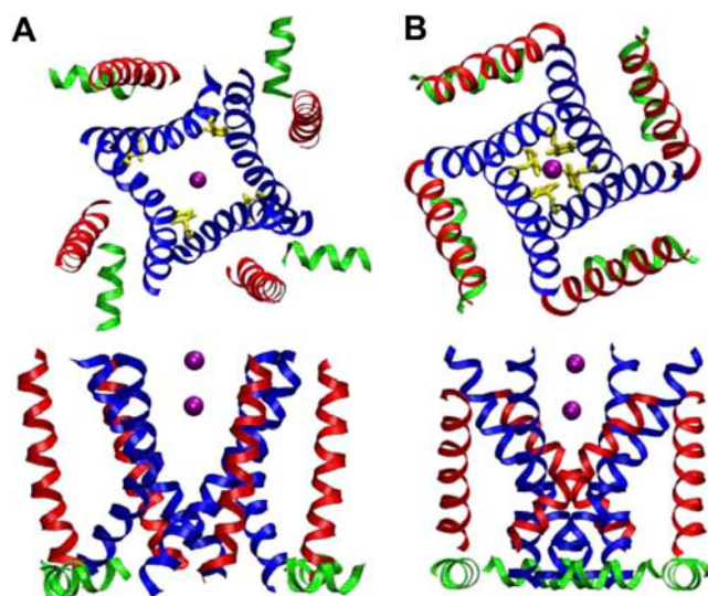
FIGURE 1 Schematic diagrams of the open (A) and closed (B) conformers of KirBac1.1. In panels A and B top figures, the view is down the pore axis, from the extracellular end of the protein. Phe-146 activation gate is displayed as yellow sticks. In panels A and B bottom figures, the view is perpendicular to the pore axis, with the extracellular mouth at top of the diagram. The slide helices (green), inner (blue), and outer (red) helices are represented as ribbons. Purple spheres represent K^+ .
